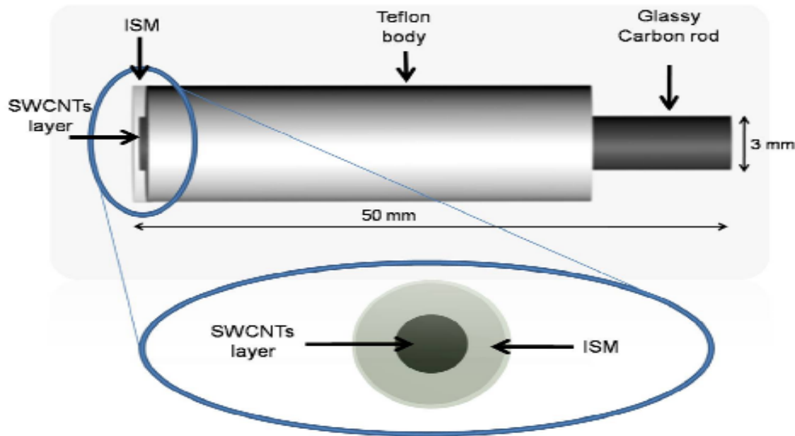
Figure 2. Scheme of the ion-selective electrode developed in our laboratory.
